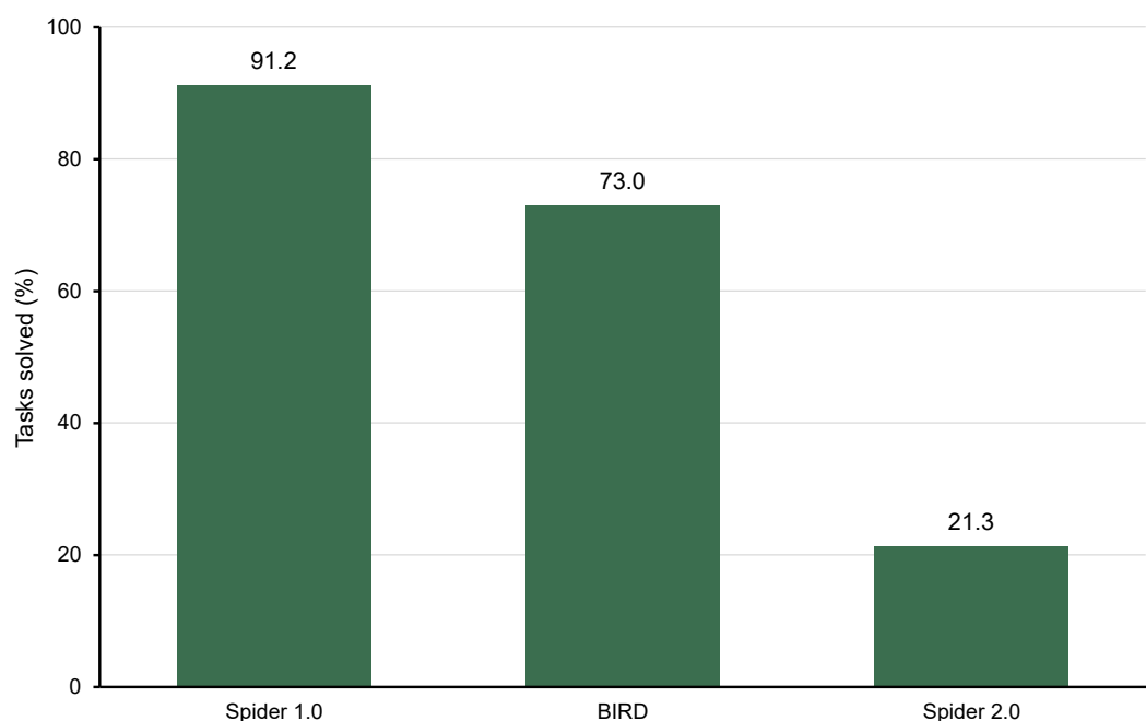
Figure 2. Share of tasks solved by the o1-preview-based Code Agent on Spider 1.0, BIRD, and Spider 2.0. Source: [3].
