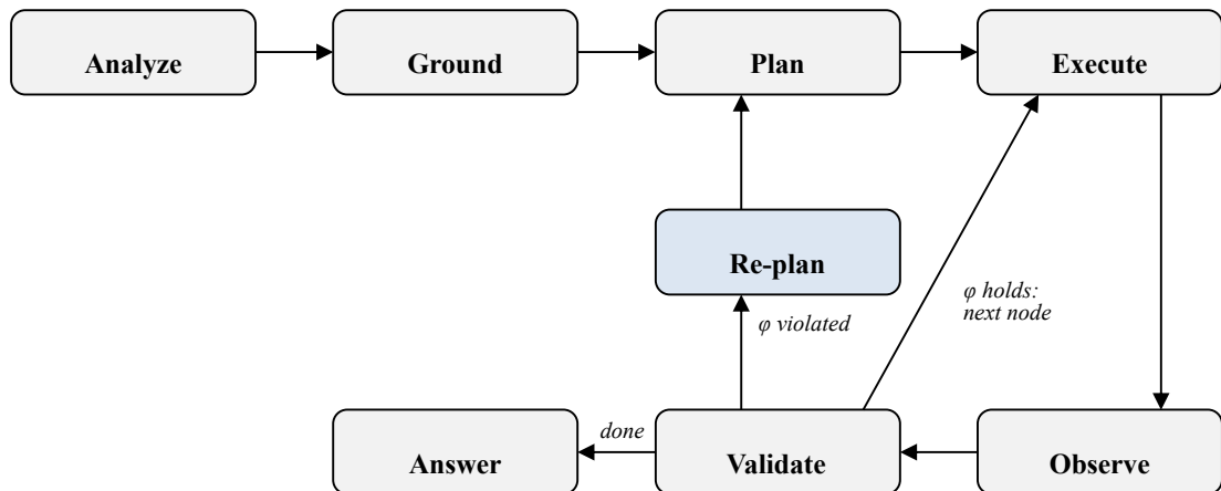
Figure 1. Architecture of LLM-driven query planning. When all nodes have been executed and validated, Validate passes control to Answer. After each validated step, control returns to Execute for the next ready node; a violated predicate \phi sends control to Re-plan, which regenerates only the unexecuted part of the plan.
